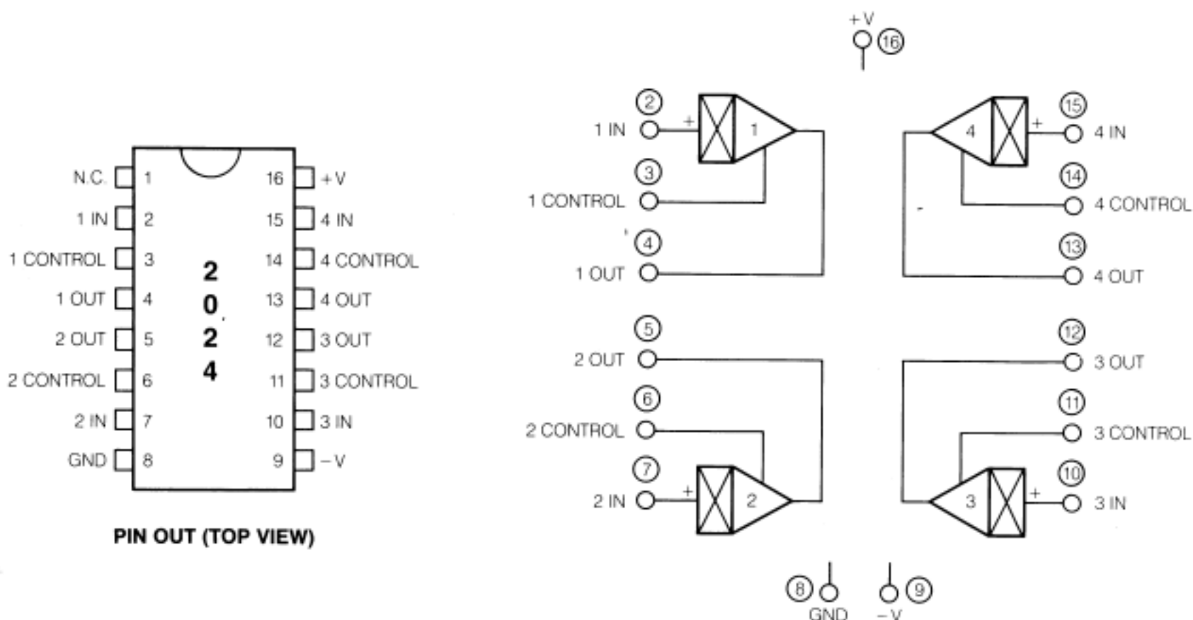
FIGURE 1. BLOCK DIAGRAM
