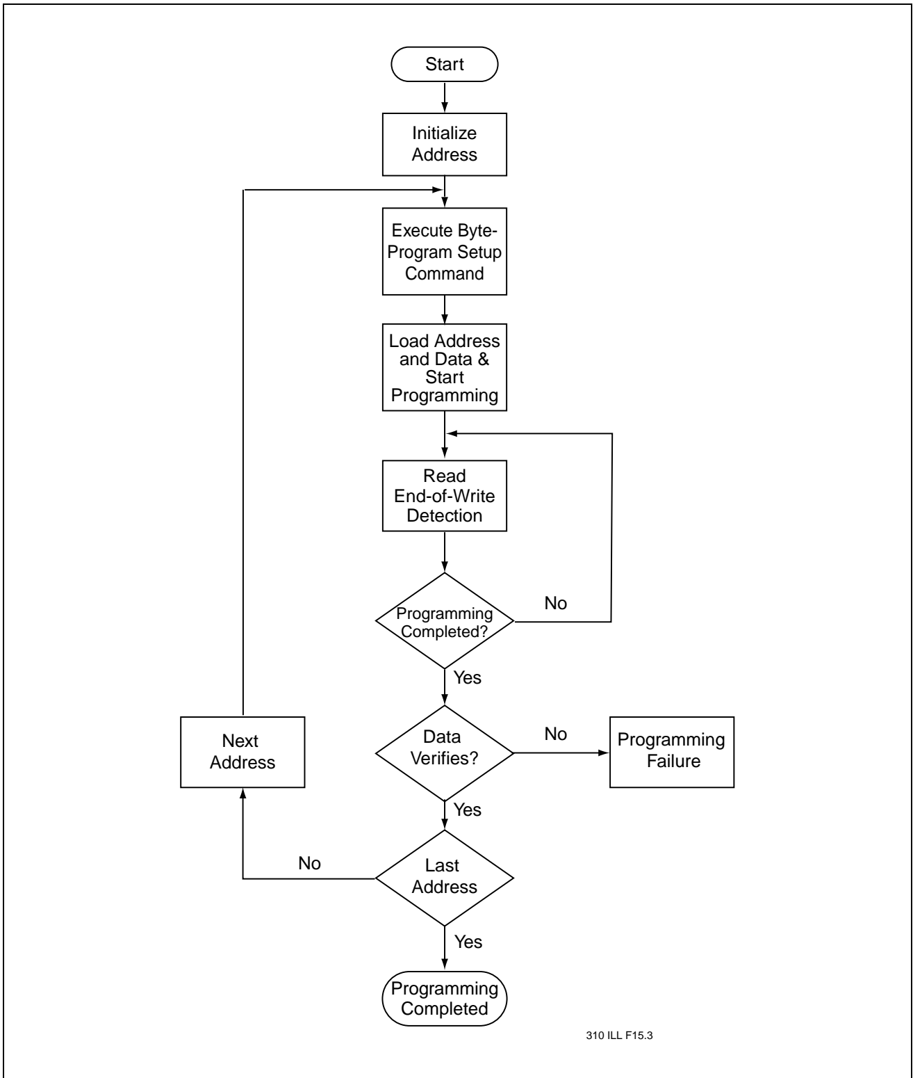
FIGURE 16: BYTE-PROGRAM FLOWCHART
