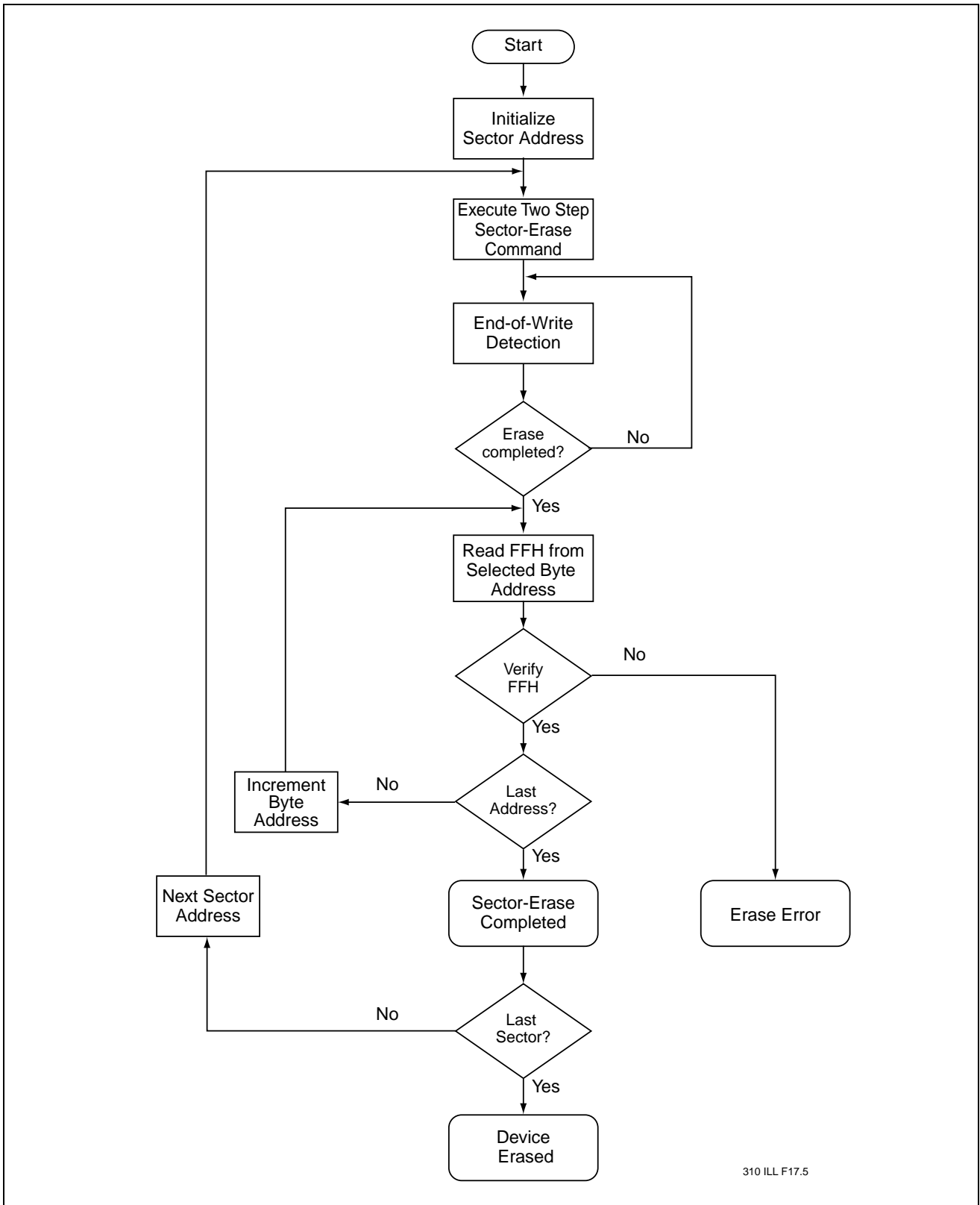
FIGURE 18: SECTOR-ERASE FLOWCHARTS
