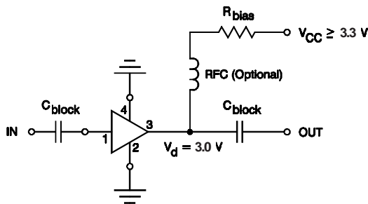
Typical Biasing Configuration
