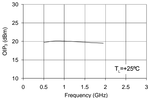
OIP 3 vs. Frequency V_D = 2.6\text{ V} , I_D = 20\text{ mA}
