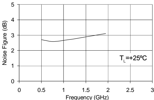
Noise Figure vs. Frequency V_D = 2.6\text{ V} , I_D = 20\text{ mA}
