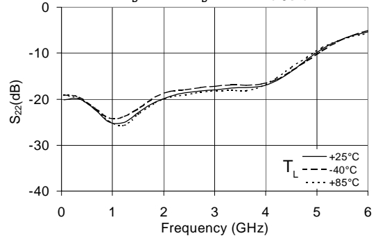
|S_{22}| vs. Frequency
