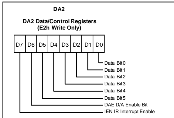
Figure 51. DA2 Data/Enable Register
