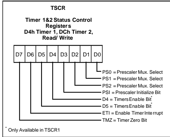
Figure 30. Timer Status Control Registers
