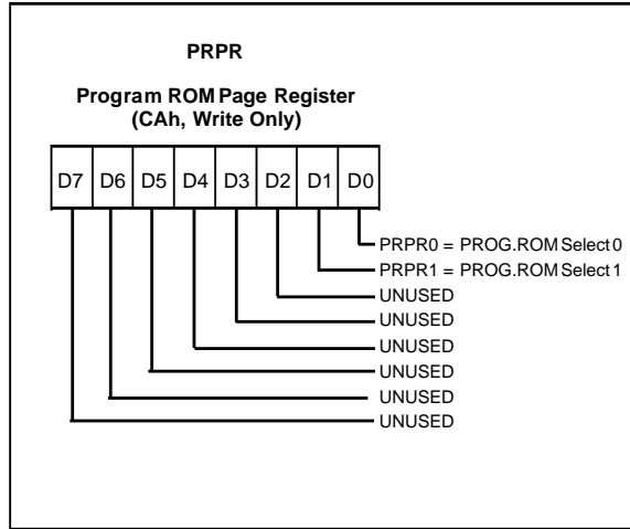
Figure 11. Program ROM Page Register
