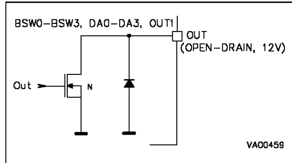
Figure 54. BSW, DA, OUT1 Output Configuration Diagram
