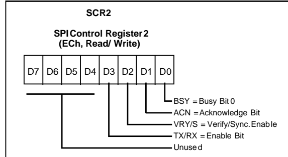
Figure 38. SPI Control Register 2
