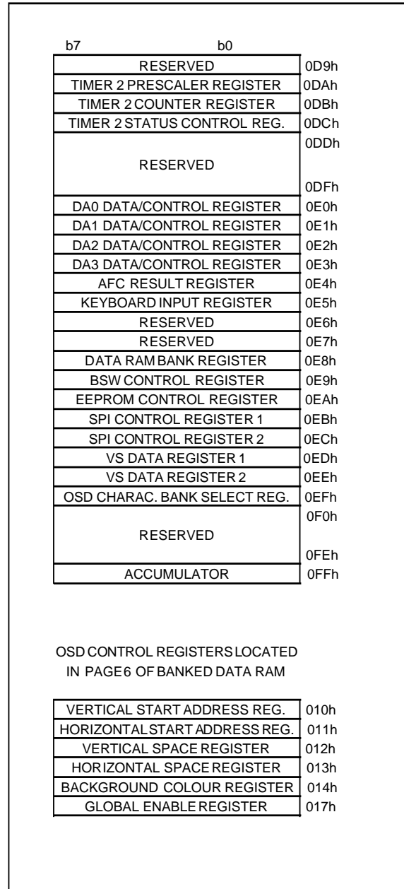
Figure 13. ST631xx Data Space (Continued)
