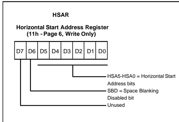
Figure 63. Horizontal Start Address Register
