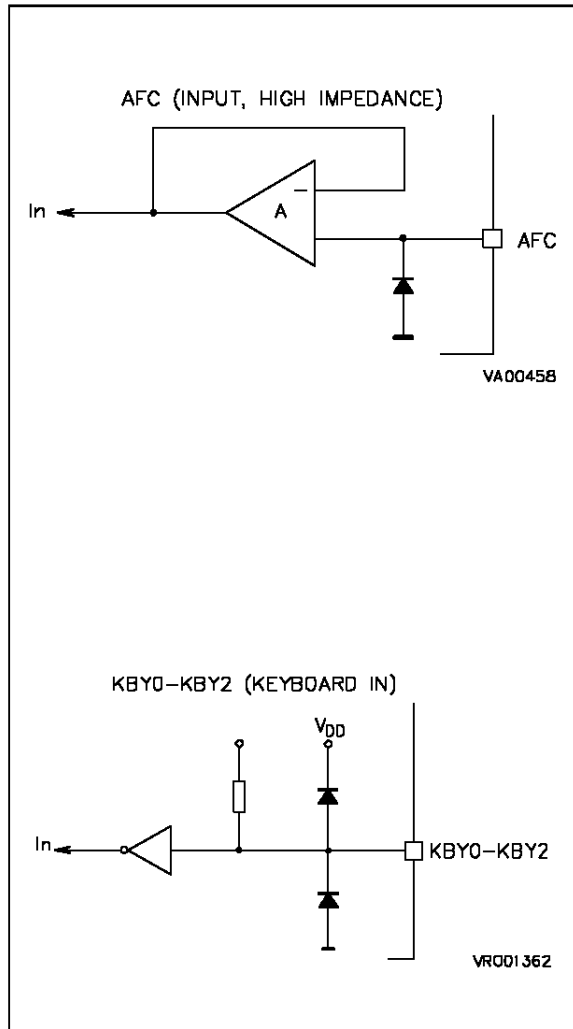
Figure 53. AFC, KBY Inputs Configuration Diagrams
