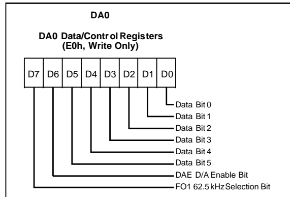
Figure 49. DA0 Data/Enable Register
