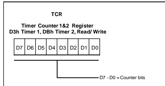
Figure 31. Timer Counter Registers
