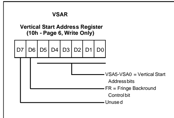
Figure 62. Vertical Start Address Register
