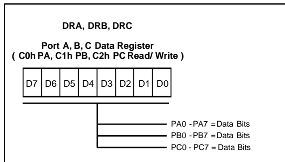
Figure 24. Port A, B, C Data Register
