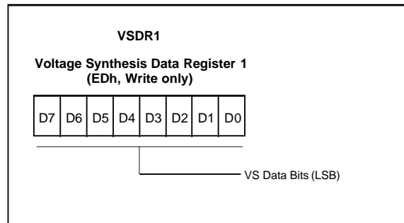
Figure 46. Voltage Synthesis Data Register 1
