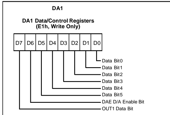
Figure 50. DA1 Data/Enable Register
