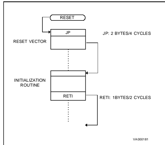
Figure 22. Restart Initialization Program Flow-Chart
