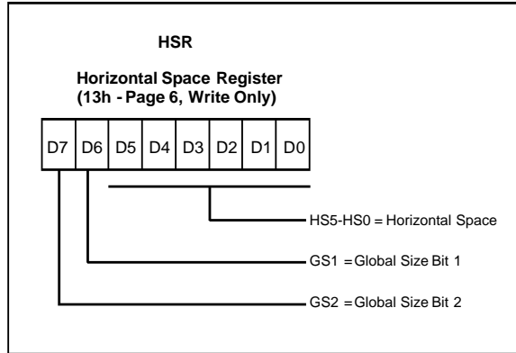
Figure 65. Horizontal Space Register
