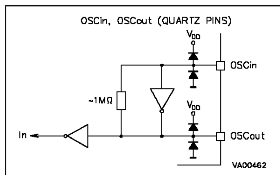
Figure 25. OSCin, OSCout Diagram
