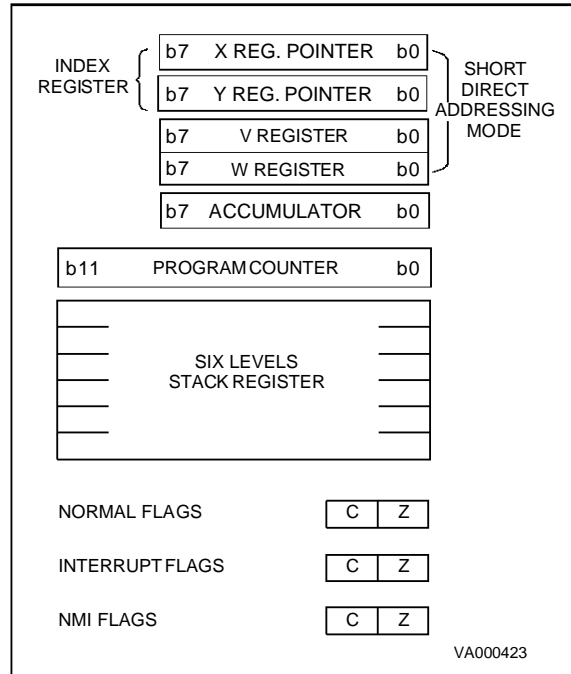
Figure 5. ST631xx Core Programming Model
