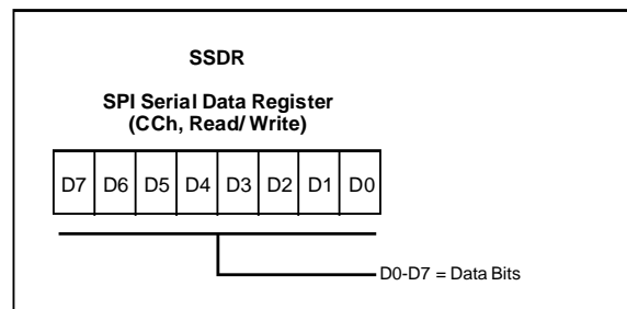
Figure 36. SPI Serial Data Register
