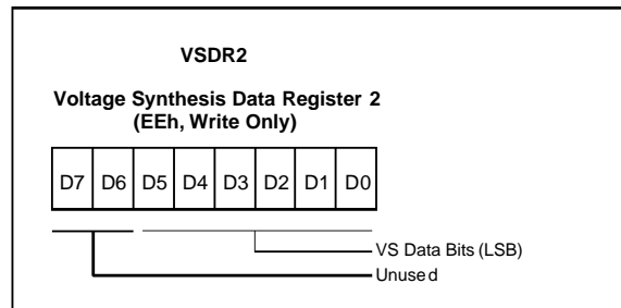
Figure 47. Voltage Synthesis Data Register 2
