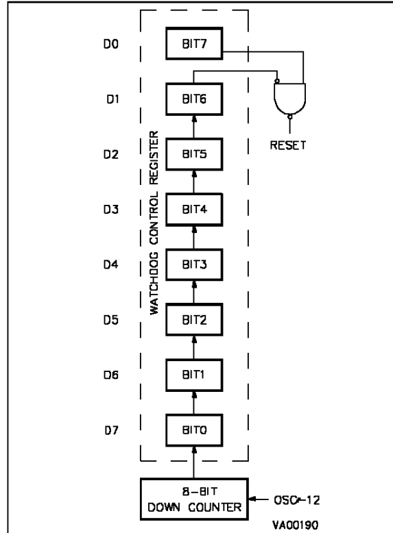
Figure 34. Hardware Activated Watchdog Working Principle
