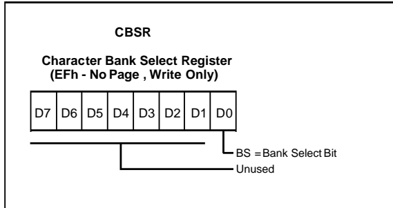
Figure 67. Character Bank Select Register
