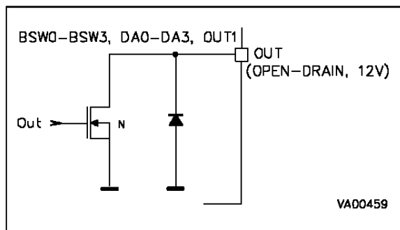
Figure 48. 6-bit PWM D/A & 62.5kHz Output Configuration
