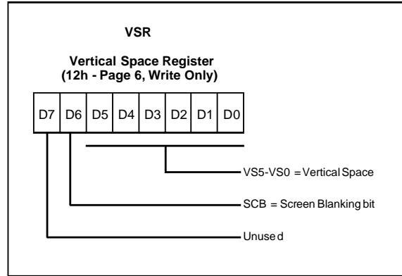
Figure 64. Vertical Space Register
