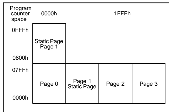
Figure 8. ST631xx 8K Bytes Program Space Addressing Description
