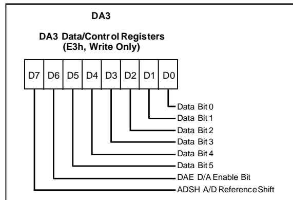
Figure 52. DA3 Data/Enable Register
