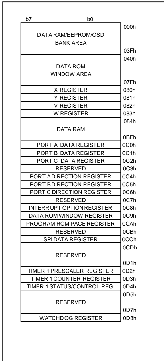
Figure 12. ST631xx Data Space
