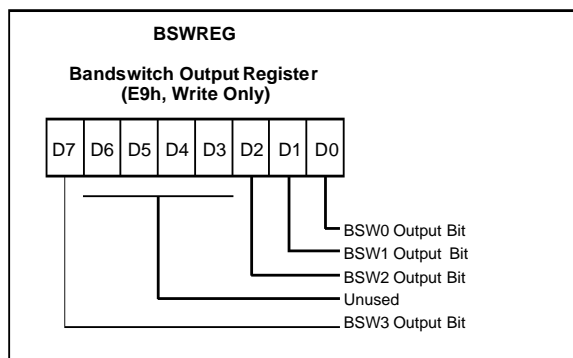
Figure 57. Bandswitch Output Register
