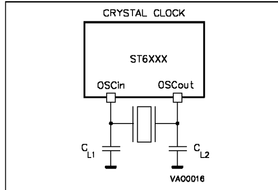
Figure 23. Clock Generator Option (1)
