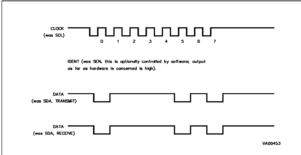
Figure 45.STD Bus (Hardware Bus Disabled) Timing Diagram
