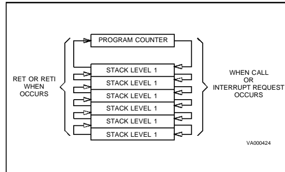
Figure 6. Stack Operation
