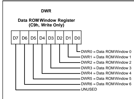
Figure 14. Data ROM Window Register
