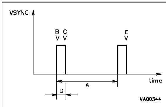
Figure 68. OSD Oscillator ON/OFF Timing
