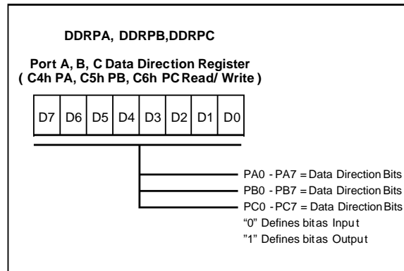
Figure 25. Port A, B, C Data Direction Register
