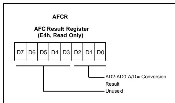
Figure 55. AFC Result Register
