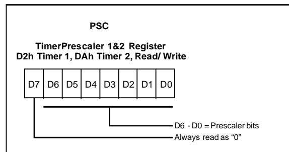
Figure 32. Timer Counter Registers
