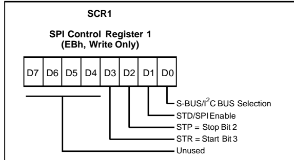
Figure 37. SPI Control Register 1
