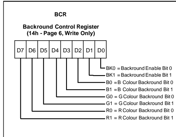
Figure 66. Background Control Register
