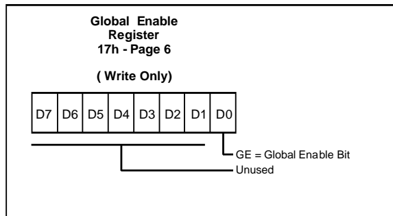
Figure 61. Global Enable Bit
