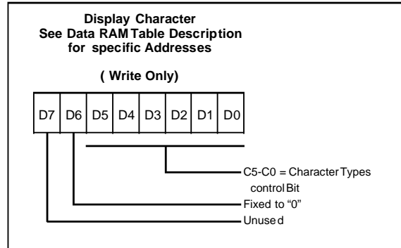
Figure 60. Display Character Register Explanation
