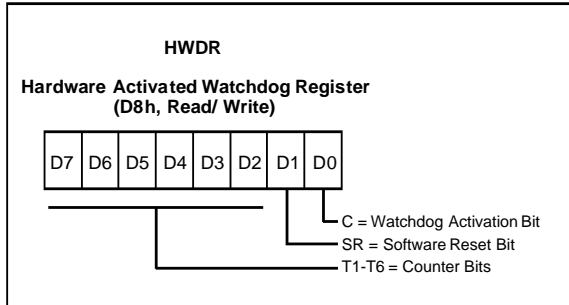
Figure 35. Watchdog Register
