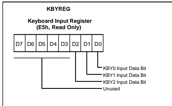
Figure 56. Keyboard Input Register
