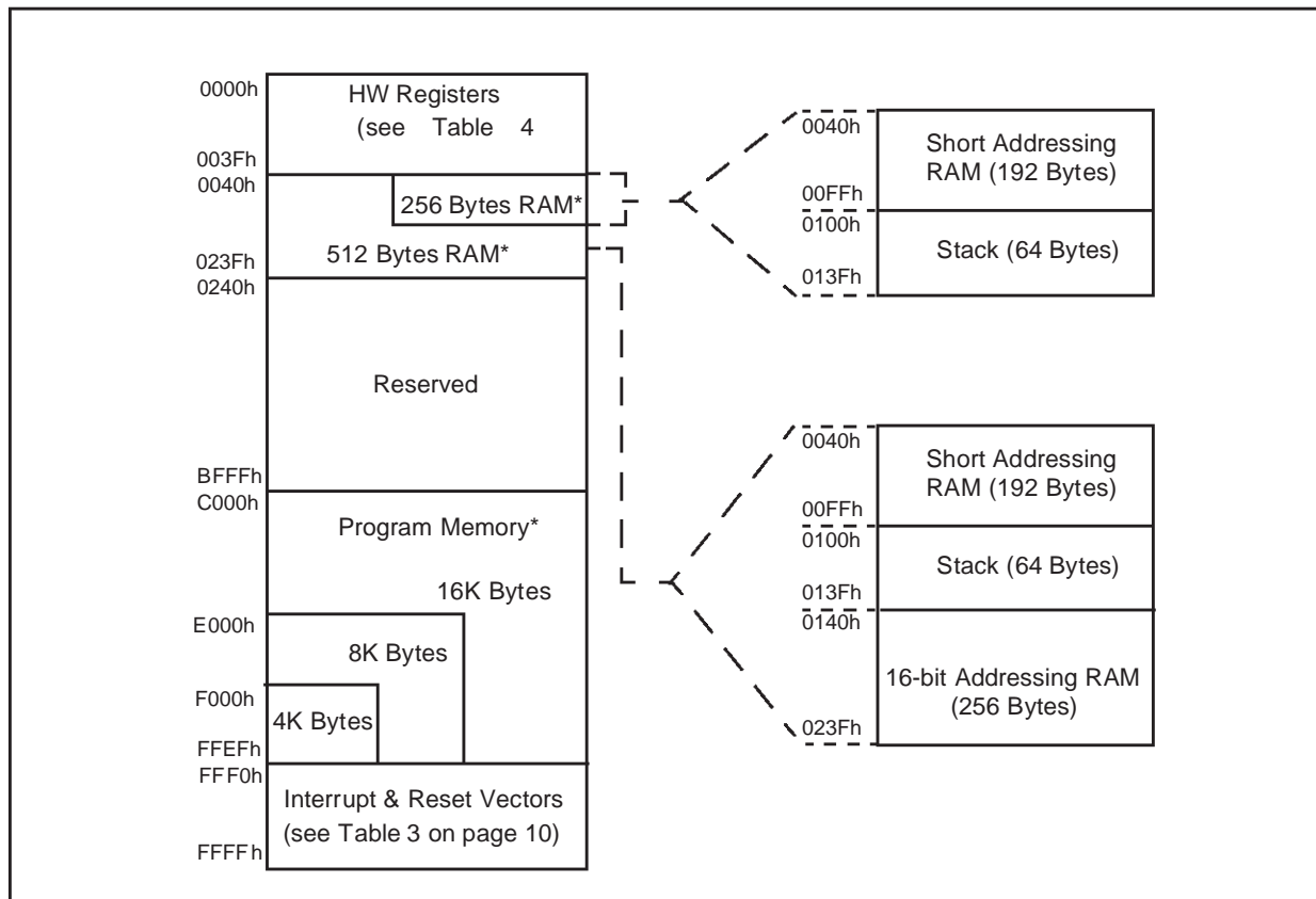
Figure 5. Memory Map
