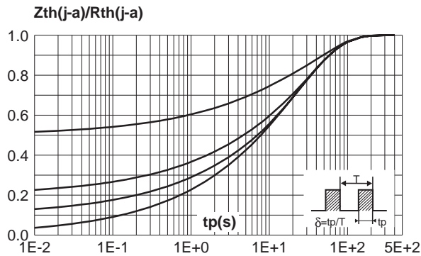
Fig. 4-1: Relative variation of thermal impedance junction to ambient versus pulse duration (epoxy printed circuit board, \epsilon(\text{Cu})=35\mu\text{m} , recommended pad layout) (SMB).
