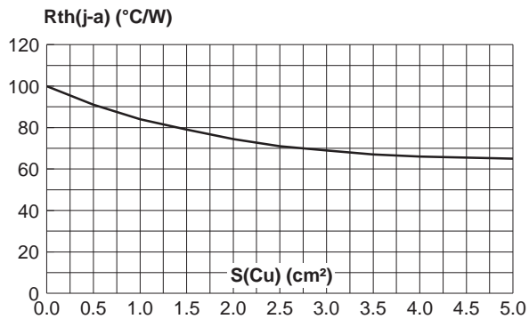
Fig. 8-1: Thermal resistance junction to ambient versus copper surface under each lead (Epoxy printed circuit board FR4, copper thickness: 35µm) (SMB).
