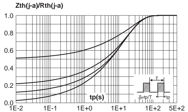
Fig. 4-2: Relative variation of thermal impedance junction to ambient versus pulse duration (epoxy printed circuit board, \epsilon(\text{Cu})=35\mu\text{m} , recommended pad layout) (SMA).
