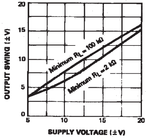
OUTPUT SWING
