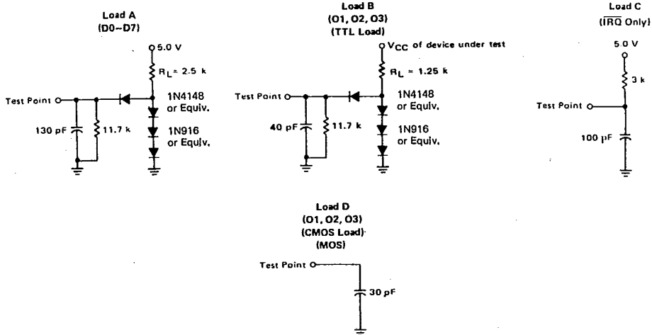
FIGURE 10 - BUS TIMING TEST LOADS
