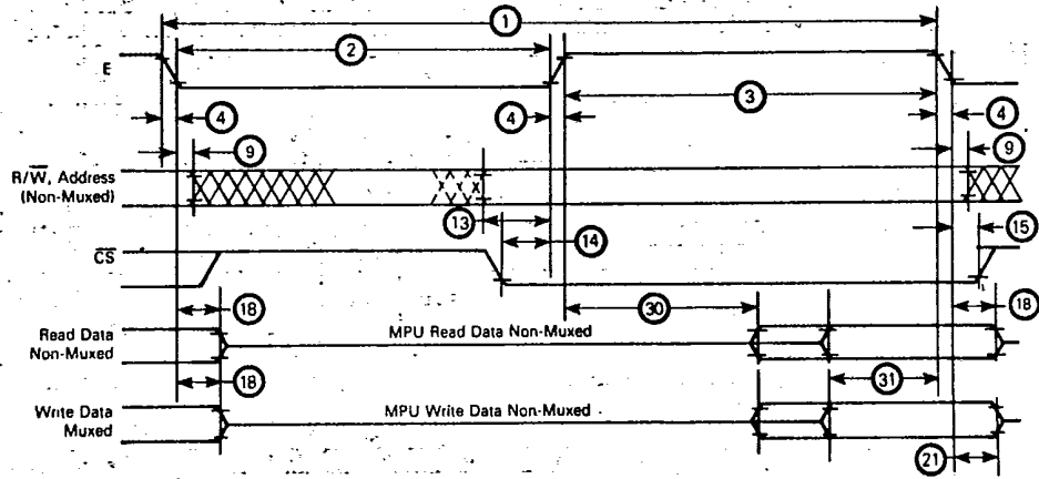
FIGURE 3 - BUS TIMING
