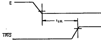
FIGURE 8 - \overline{IRQ} RELEASE TIME
