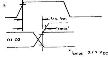
FIGURE 7 - OUTPUT DELAY
