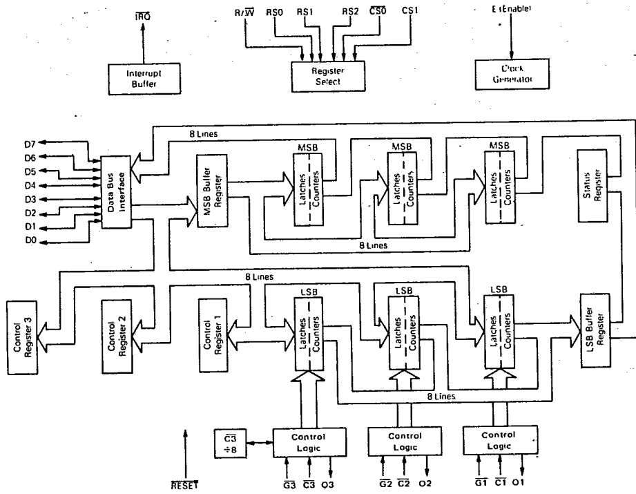
87D 09432 D T-51-19 FIGURE 2 - BLOCK DIAGRAM
