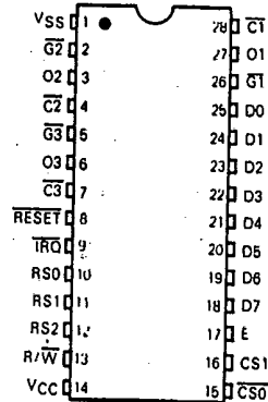
FIGURE 1 - PIN ASSIGNMENT
