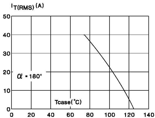
Fig.5 : RMS on-state current versus case temperature. (BTA)
