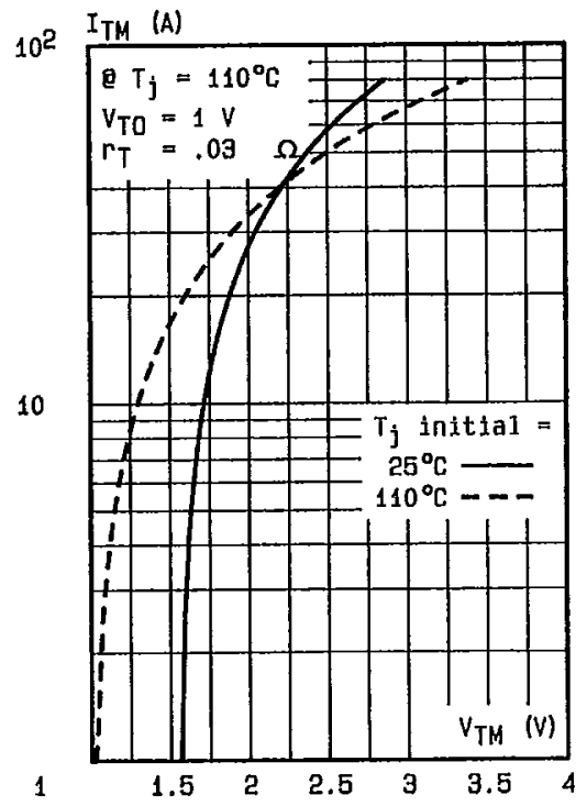
Fig.8 - On-state characteristics (maximum values).
