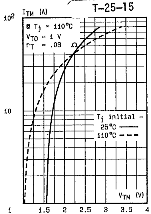
Fig.8 - On-state characteristics (maximum values).
