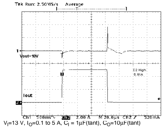
Figure 29 : Load Transient
