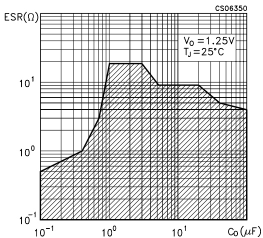
Figure 21 : Stability
