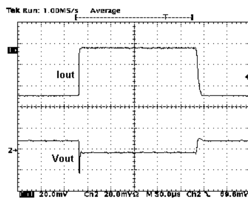
Figure 28 : Load Transient
