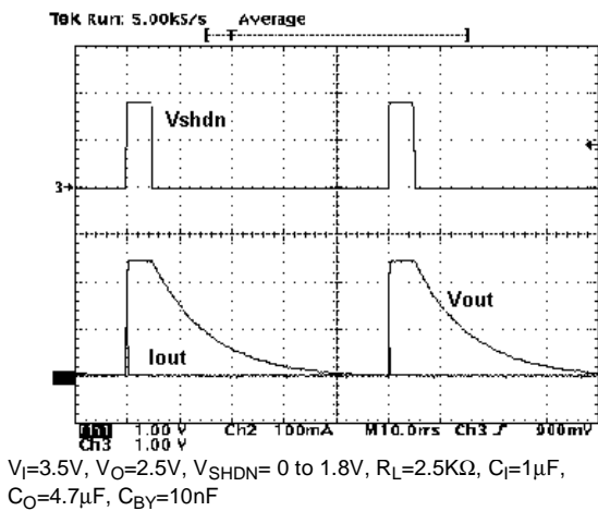
Figure 21 : Start-up Transient
