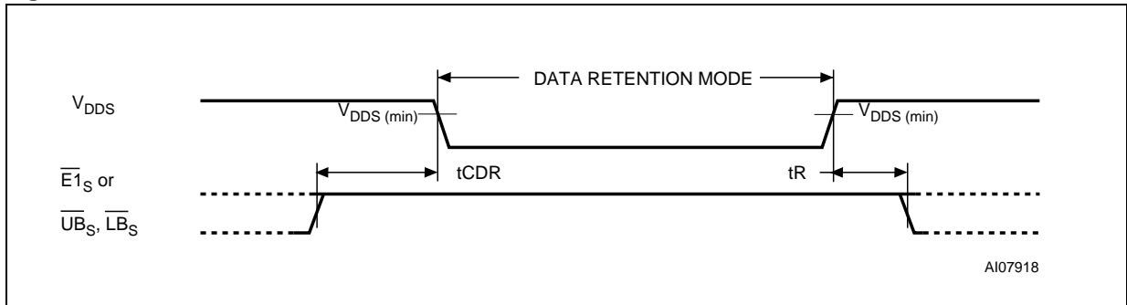
Figure 24. SRAM Low V_{DD\bar{S}} Data Retention AC Waveforms, \bar{E}1\bar{S} or \bar{U}\bar{B}\bar{S} / \bar{L}\bar{B}\bar{S} Controlled
