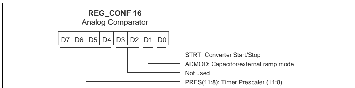
Figure 7.5 Configuration Register 16
