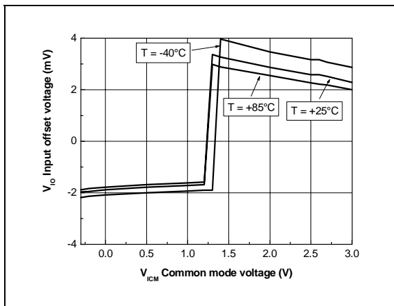
V_{IO} vs V_{ICM} & Temperature @ V_{CC}=10V
