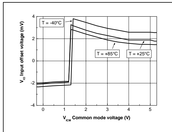
V_{IO} vs V_{ICM} & Temperature @ V_{CC}=5V
