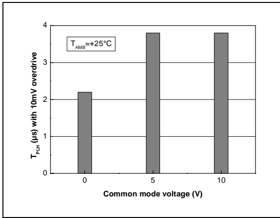
T_{PLH} vs V_{ICM} @ V_{CC}=5V and 10mV overdrive
