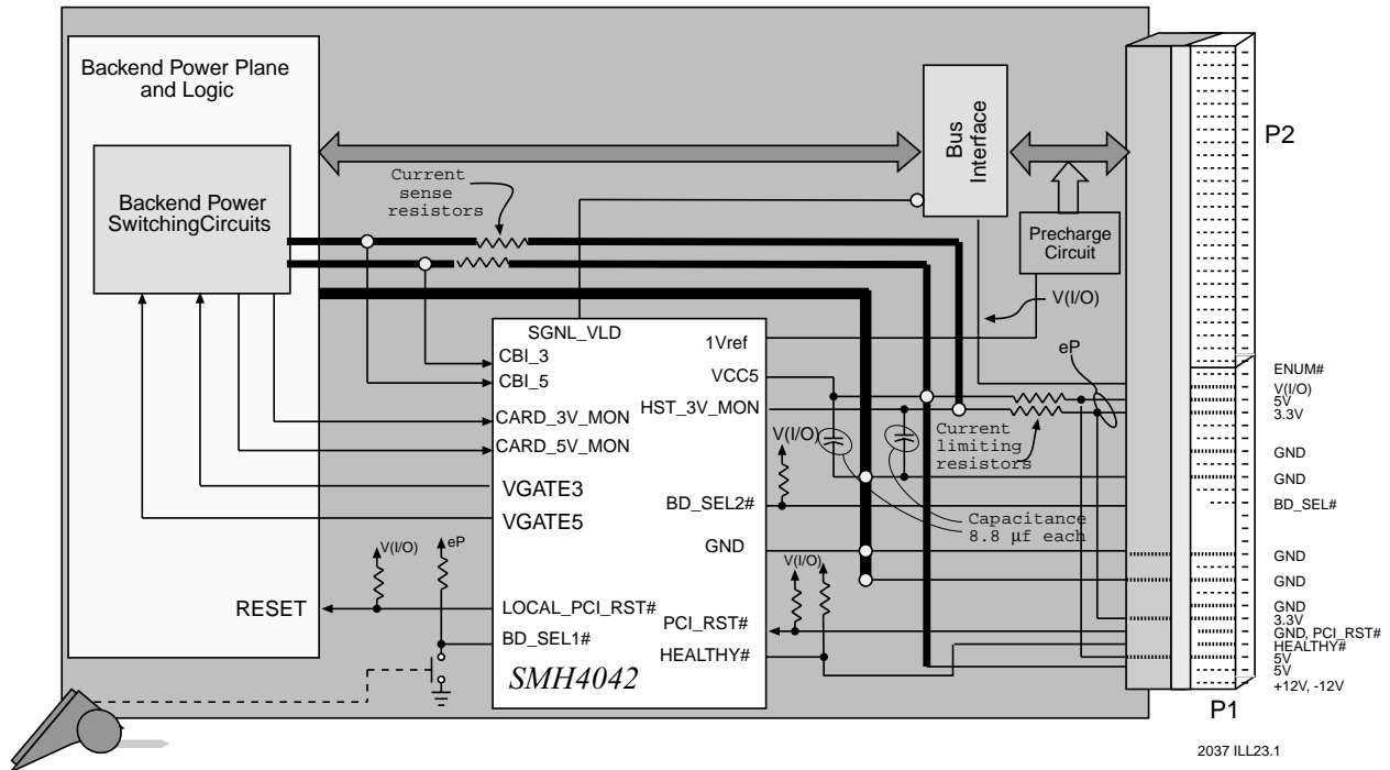
Figure 2. Block diagram of typical CompactPCI board.
