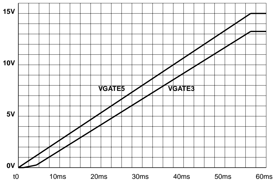
Figure 4. Typical delay between VGATE5 and VGATE3
