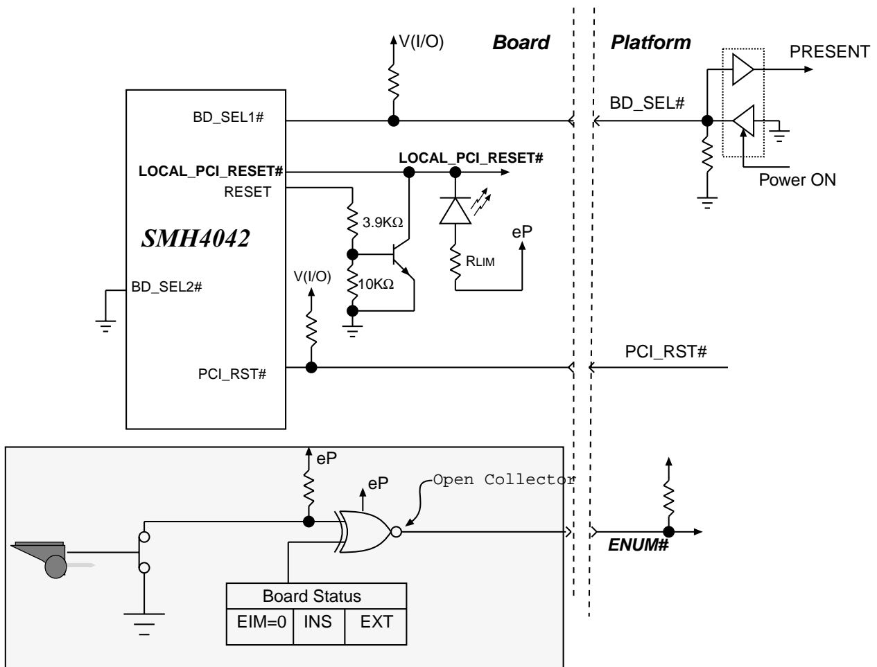
Figure 9. Full HotSwap board/host interface
