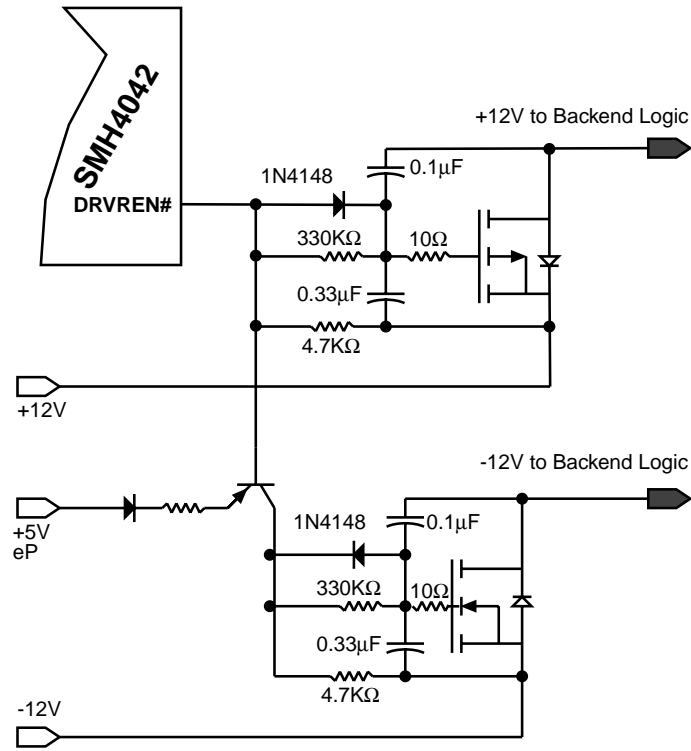
Figure 10. Using DRVREN# to switch + and -12V to the backend logic
