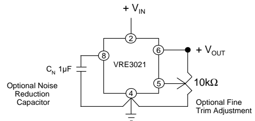
Figure 3 External Connections
