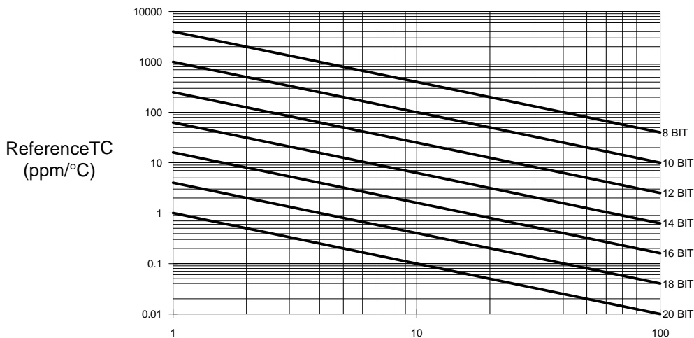
Reference TC vs. ΔT change from 25°C for 1 LSB change
