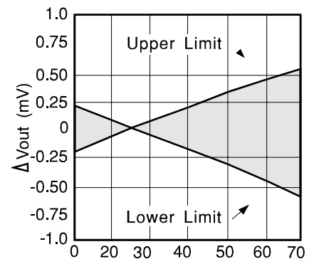
Temperature °C VRE304C
