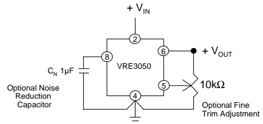
Figure 3 External Connections
