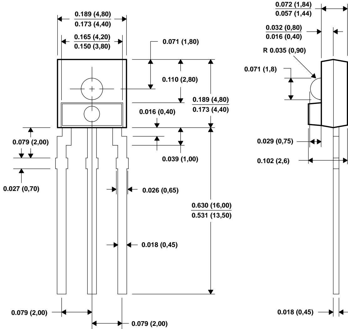
Figure 7. Package Configuration
