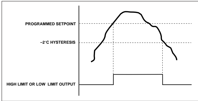
Figure 3. High Set and Low Set Thresholds
