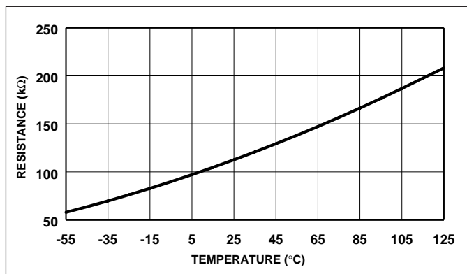
Figure 1. TC623 Sense Resistors vs. Trip Temperature
