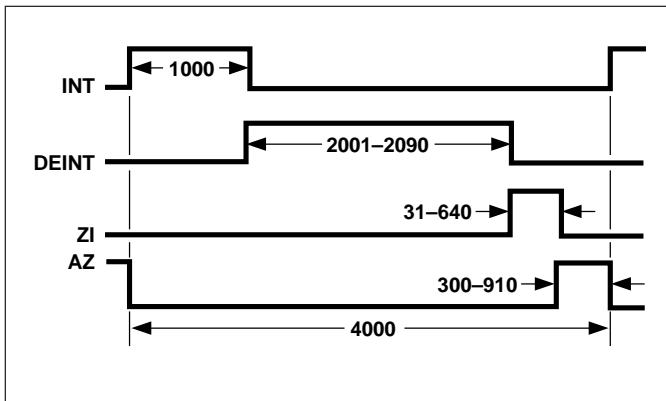
Figure 5. Conversion Timing During Overrange Operation
