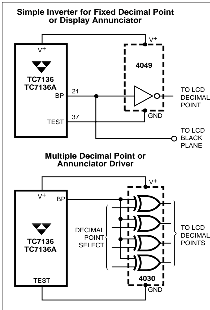
Figure 11. Decimal Point and Annunciator Drives
