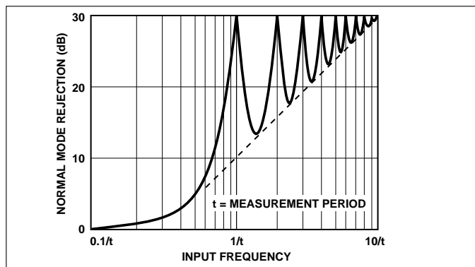
Figure 2. Normal-Mode Rejection of Dual-Slope Converter
