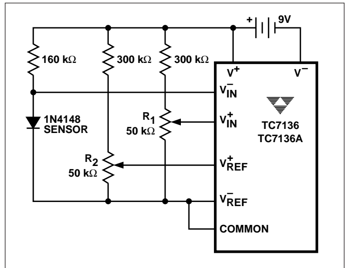
Figure 13. Temperature Sensor
