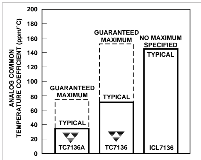
Figure 9. Analog Common Temperature Coefficient
