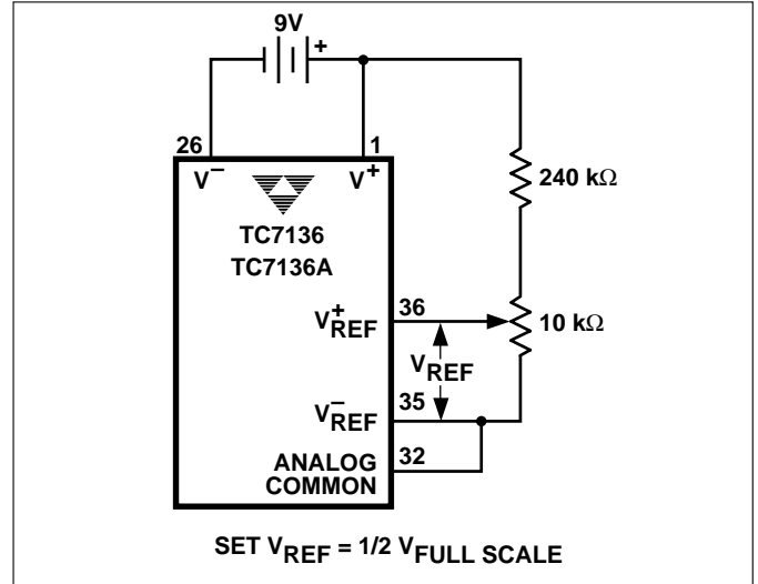
Figure 10. TC7136A Internal Voltage Reference Connection
