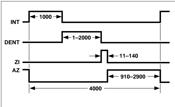
Figure 4. Conversion Timing During Normal Operation
