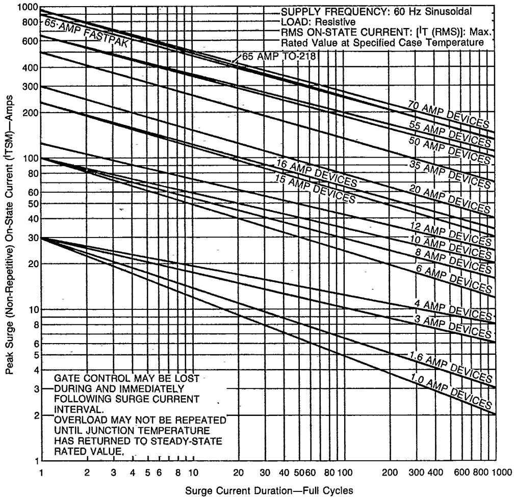
FIGURE 9 — Peak Surge Current vs Surge Current Duration
