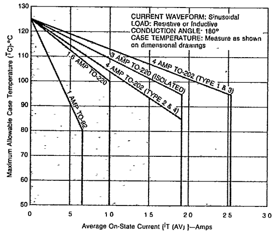
FIGURE 3A — Maximum Allowable Case Temperature vs Average On-State Current
