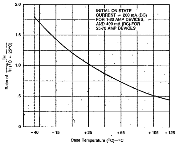
FIGURE 4 — Normalized DC Holding Current vs Case Temperature
