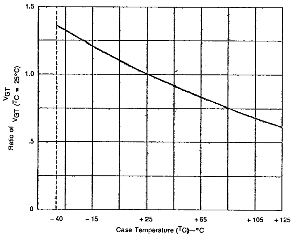
FIGURE 7 — Normalized DC Gate-Trigger Voltage vs Case Temperature
