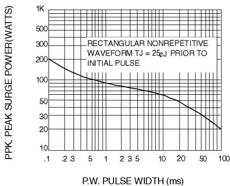
Fig. 3-MAXIMUM SURGE POWER
