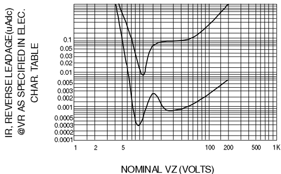
Fig. 4-TYPICAL REVERSE LEAKAGE
