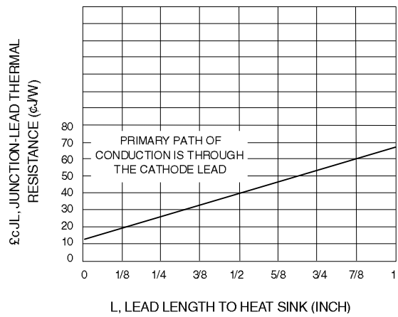
Fig. 10-TYPICAL THERMAL RESISTANCE
