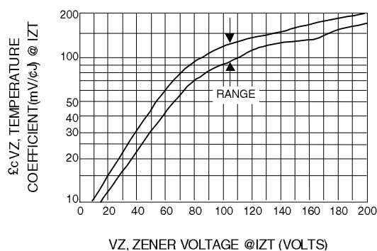
Fig. 6-UNITS 10 TO 200 VOLTS
