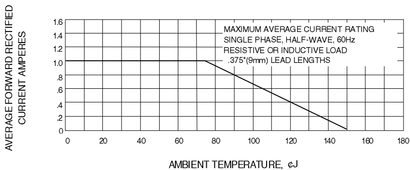
Fig. 5-FORWARD DERATING CURVE
