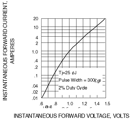
Fig. 1-TYPICAL FORWARD CHARACTERISTICS
