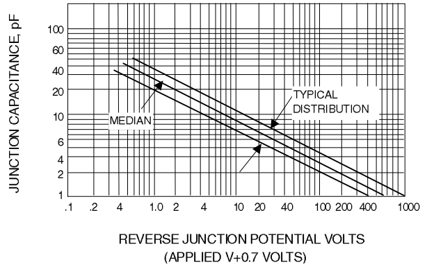
Fig. 2-JUNCTION CAPACITANCE
