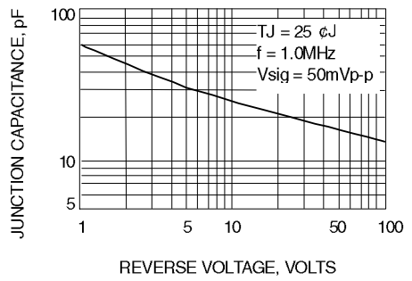
Fig. 4-TYPICAL JUNCTION CAPACITANCE
