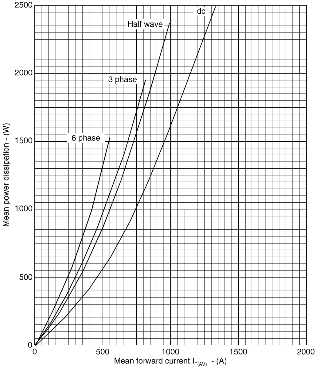
Fig. 2 Dissipation curves
