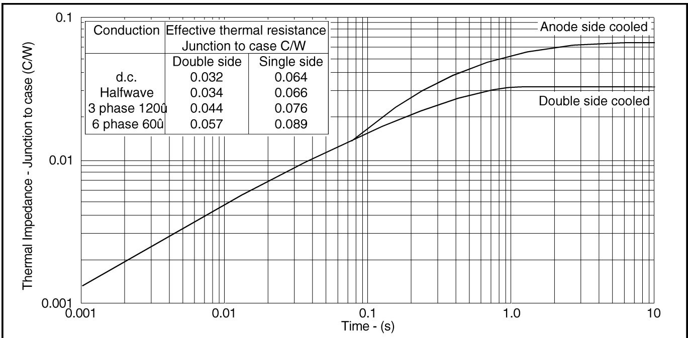
Fig. 6 Transient thermal impedance - junction to case - (C/W)
