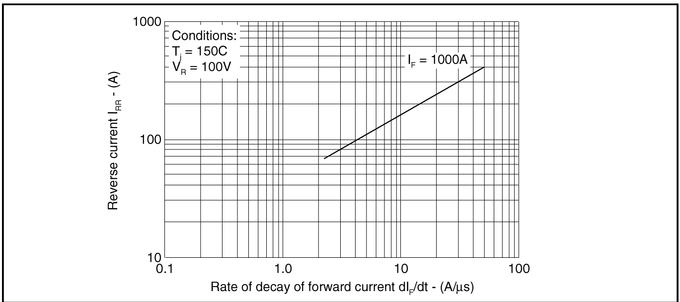
Fig. 4 Maximum reverse recovery current
