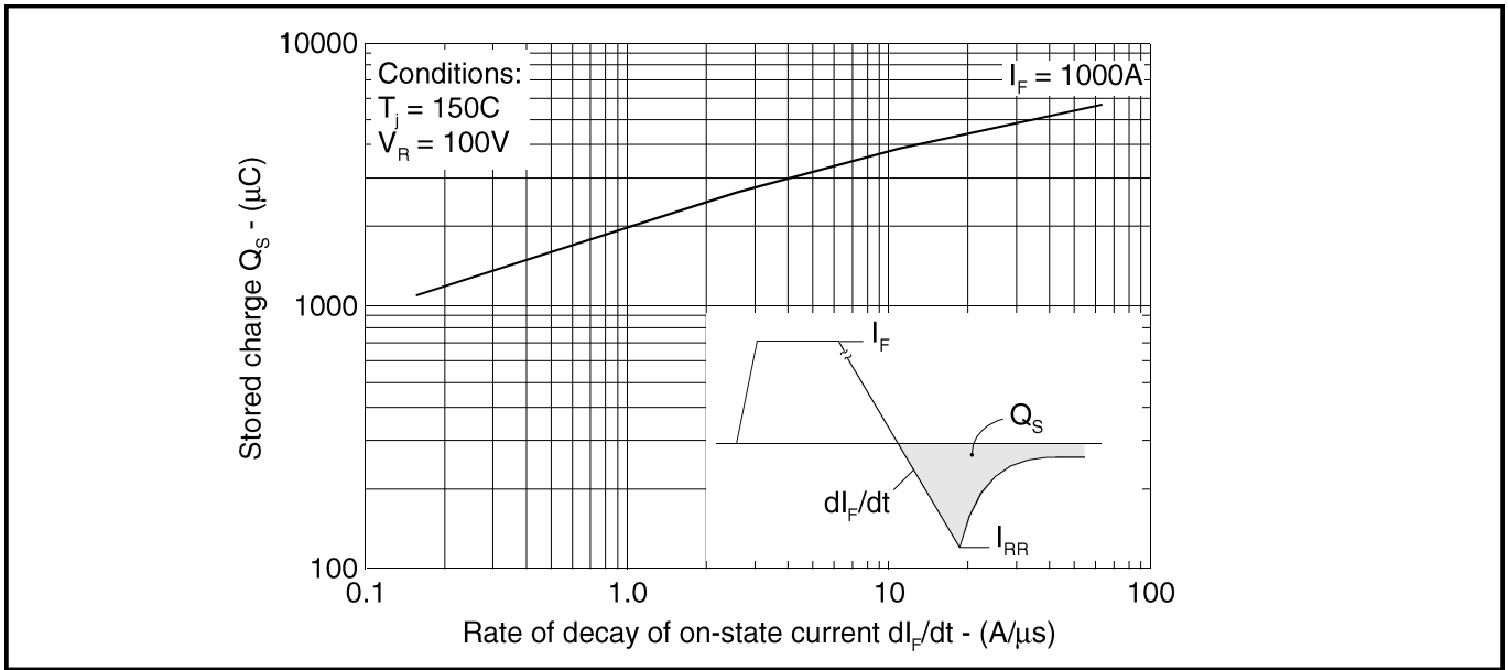
Fig. 3 Maximum total stored charge
