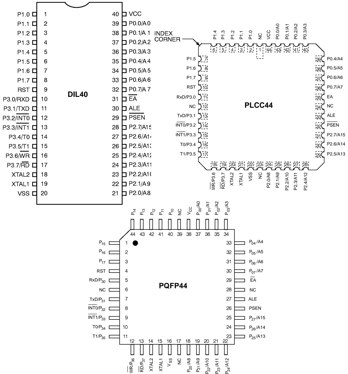
Figure 2. Pin Configuration
