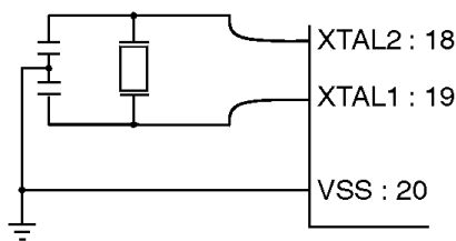
Figure 5. Crystal Oscillator.
