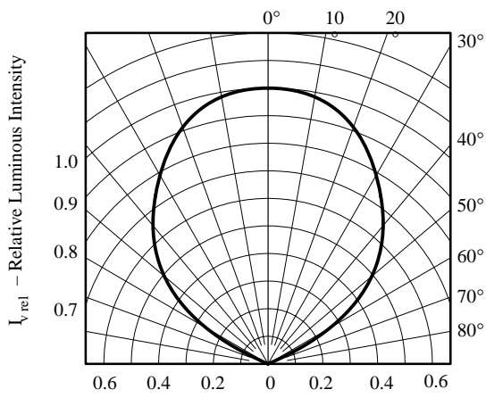
95 10082 Figure 3. Rel. Luminous Intensity vs. Angular Displacement
