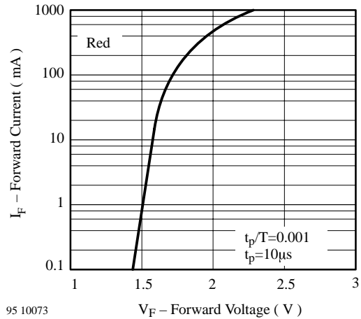
95 10073 V_F – Forward Voltage (V) Figure 4. Forward Current vs. Forward Voltage
