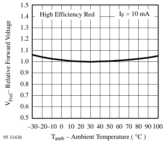
Figure 3 Relative Forward Voltage vs. Ambient Temperature
