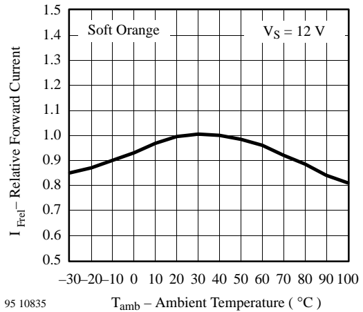
Figure 8 Relative Forward Current vs. Ambient Temperature
