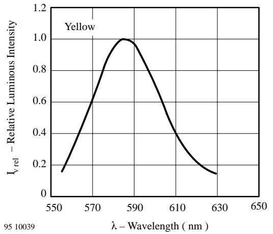
95 10039 Figure 14 Relative Luminous Intensity vs. Wavelength
