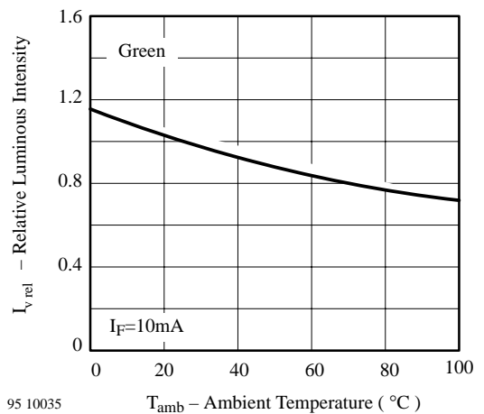
95 10035 Figure 16 Rel. Luminous Intensity vs. Ambient Temperature
