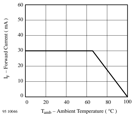
95 10046 T_{amb} - Ambient Temperature ( °C ) Figure 2 Forward Current vs. Ambient Temperature
