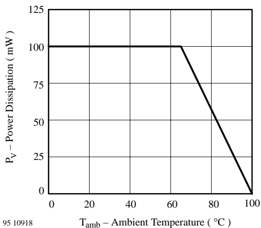
95 10918 T_{amb} - Ambient Temperature ( °C ) Figure 1 Power Dissipation vs. Ambient Temperature
