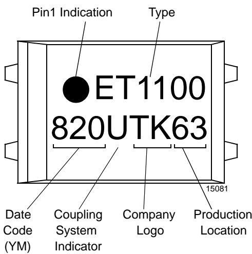
Figure 16. Marking example
