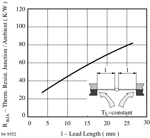
94 9552 R_{thJA} – Therm. Resist. Junction / Ambient (K/W) l – Lead Length (mm) Figure 1. Max. Thermal Resistance vs. Lead Length
