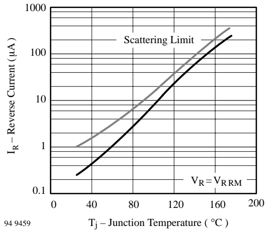
94 9459 I_R – Reverse Current ( \mu\text{A} ) T_j – Junction Temperature ( ^\circ\text{C} ) Figure 4. Reverse Current vs. Junction Temperature
