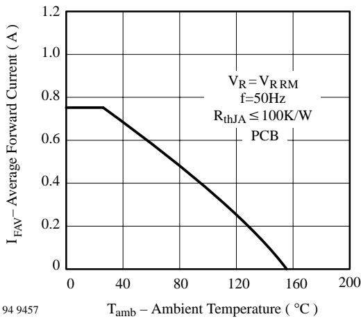
94 9457 I_{FAV} – Average Forward Current (A) T_{amb} – Ambient Temperature ( ^\circ\text{C} ) Figure 2. Max. Average Forward Current vs. Ambient Temperature
