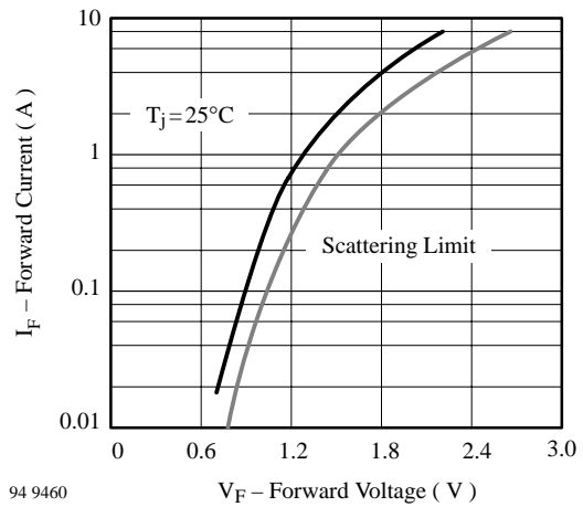
94 9460 I_F – Forward Current (A) V_F – Forward Voltage (V) Figure 5. Forward Current vs. Forward Voltage
