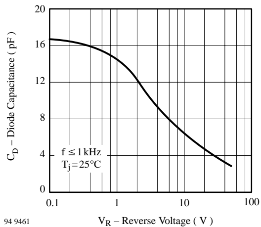
94 9461 C_D – Diode Capacitance (pF) V_R – Reverse Voltage (V) Figure 6. Typ. Diode Capacitance vs. Reverse Voltage
