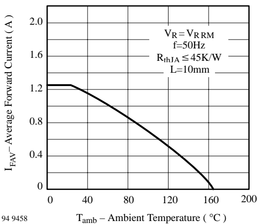
94 9458 I_{FAV} – Average Forward Current (A) T_{amb} – Ambient Temperature ( ^\circ\text{C} ) Figure 3. Max. Average Forward Current vs. Ambient Temperature
