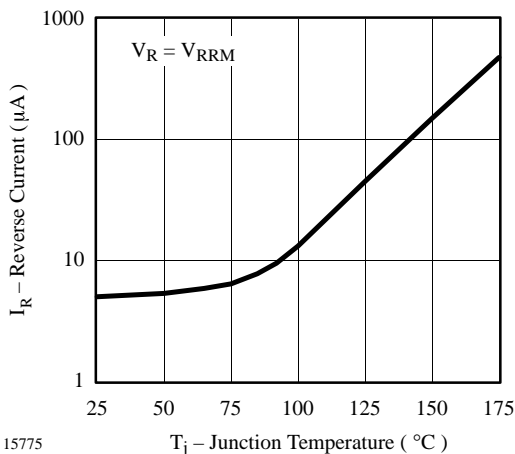
15775 Figure 3. Max. Reverse Current vs. Junction Temperature
