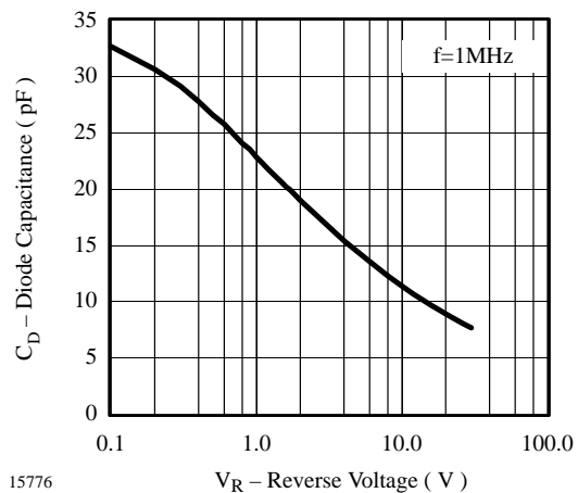
15776 Figure 6. Typ. Diode Capacitance vs. Reverse Voltage
