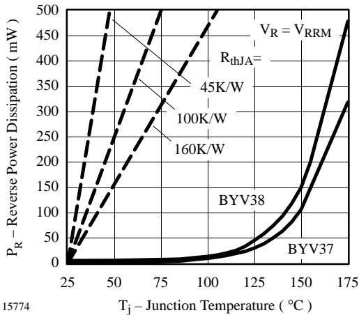
15774 Figure 2. Max. Reverse Power Dissipation vs. Junction Temperature
