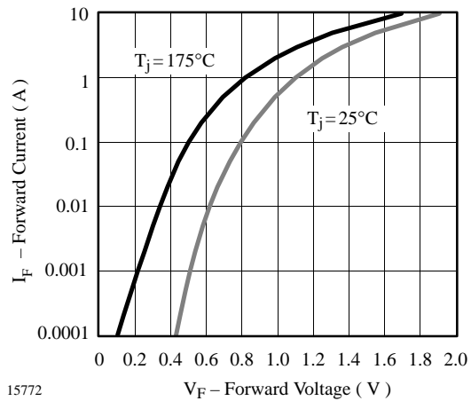
15772 Figure 5. Max. Forward Current vs. Forward Voltage
