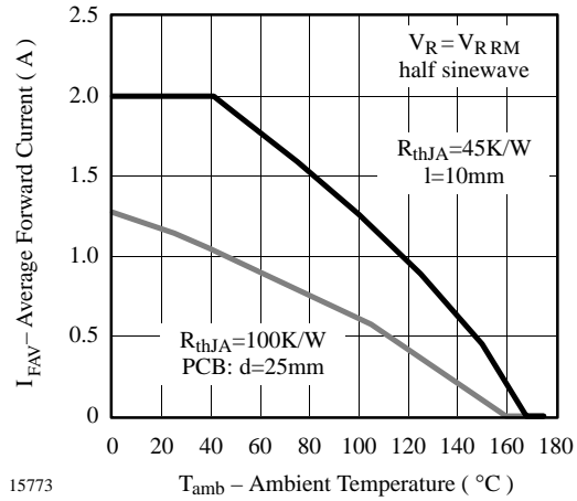
15773 Figure 4. Max. Average Forward Current vs. Ambient Temperature
