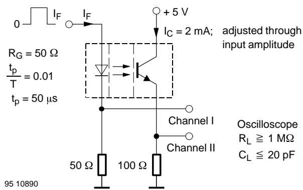
Figure 1. Test circuit
