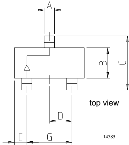
BAT54
