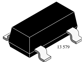
S593T Marking: 593 Plastic case (SOT 143) 1 = Source, 2 = Drain, 3 = Gate 2, 4 = Gate 1
