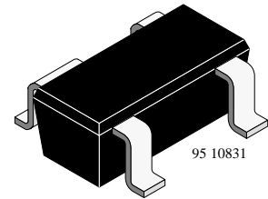
S593TR Marking: 93R Plastic case (SOT 143R) 1 = Source, 2 = Drain, 3 = Gate 2, 4 = Gate 1
