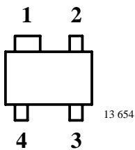
S593TRW Marking: W93 Plastic case (SOT 343R) 1 = Source, 2 = Drain, 3 = Gate 2, 4 = Gate 1
