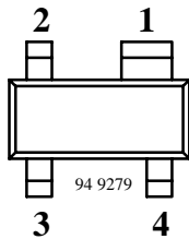
S593T Marking: 593 Plastic case (SOT 143) 1 = Source, 2 = Drain, 3 = Gate 2, 4 = Gate 1
