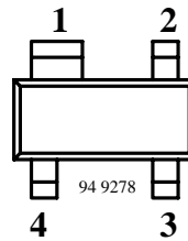
S593TR Marking: 93R Plastic case (SOT 143R) 1 = Source, 2 = Drain, 3 = Gate 2, 4 = Gate 1
