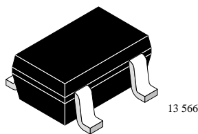
S593TRW Marking: W93 Plastic case (SOT 343R) 1 = Source, 2 = Drain, 3 = Gate 2, 4 = Gate 1
