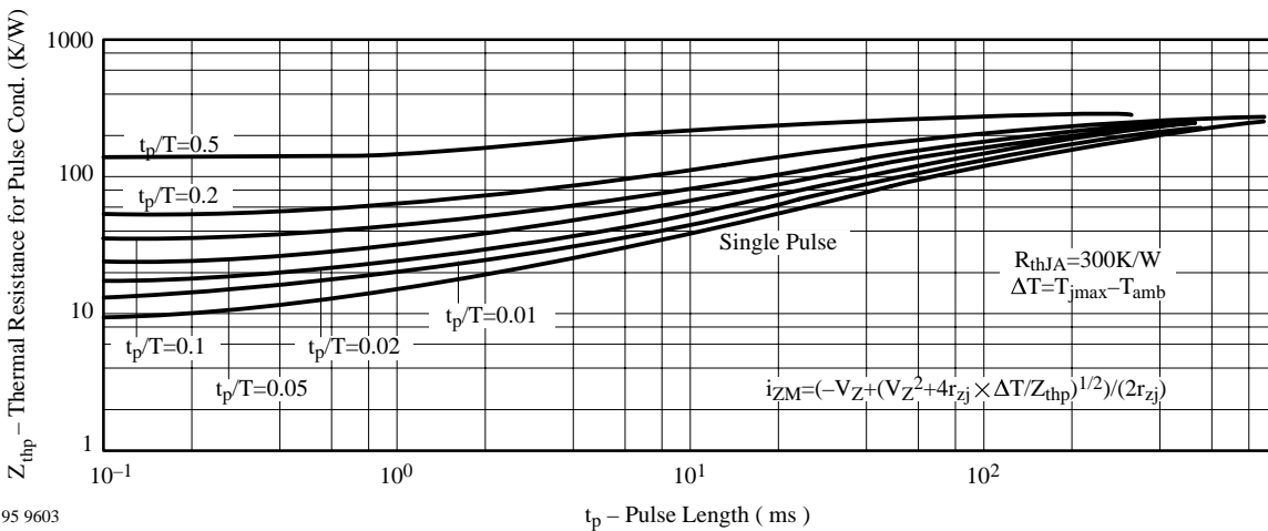
Thermal Response
