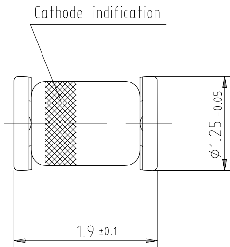
Glass case Micro MELF
