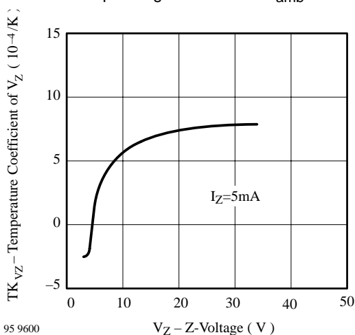
Temperature Coefficient of V_Z vs. Z-Voltage
