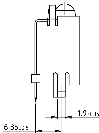
View "A"
