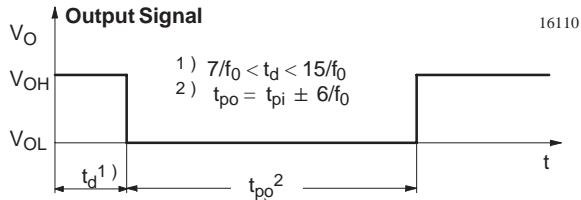
Figure 7. Output Function
