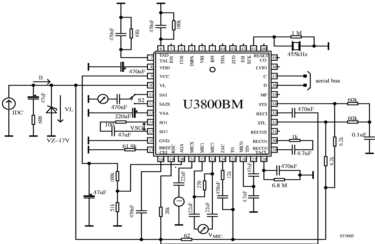
Figure 8. Test circuit
