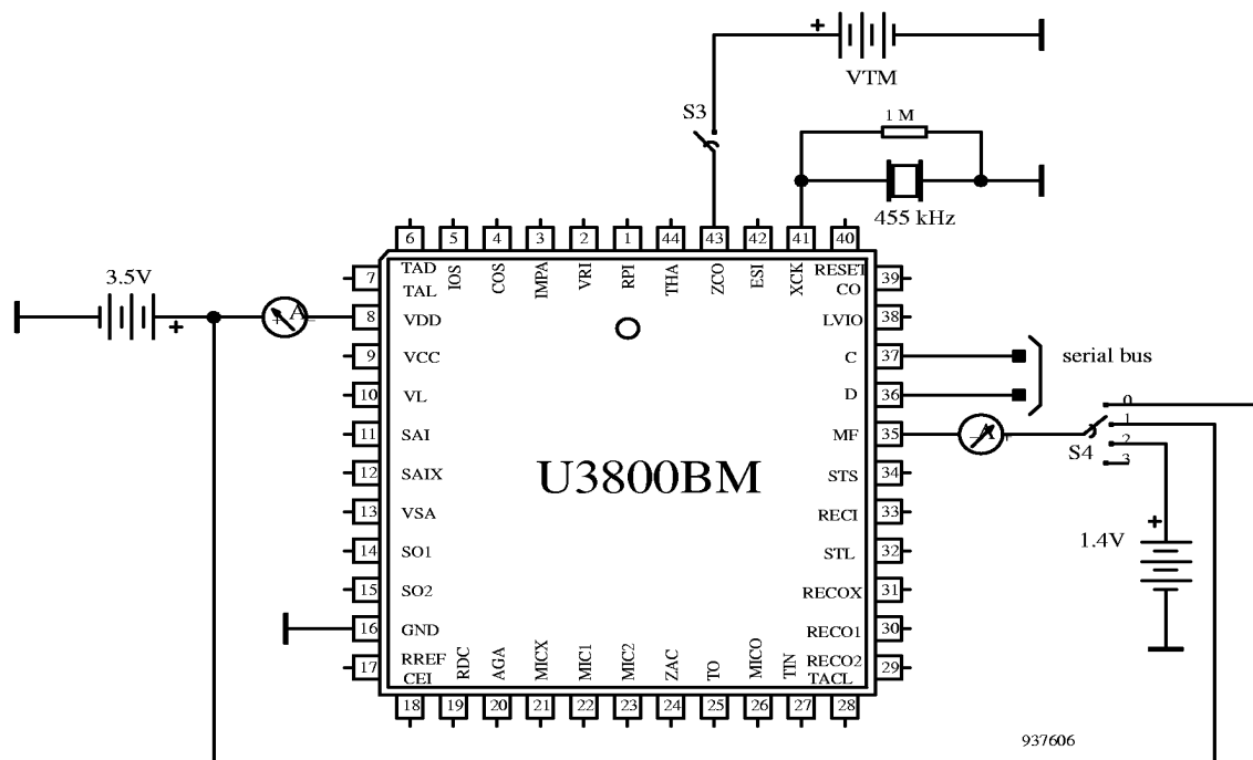
Figure 9. Test circuit
