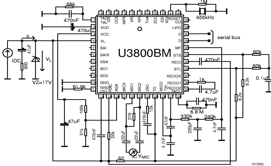
Figure 6. Test circuit
