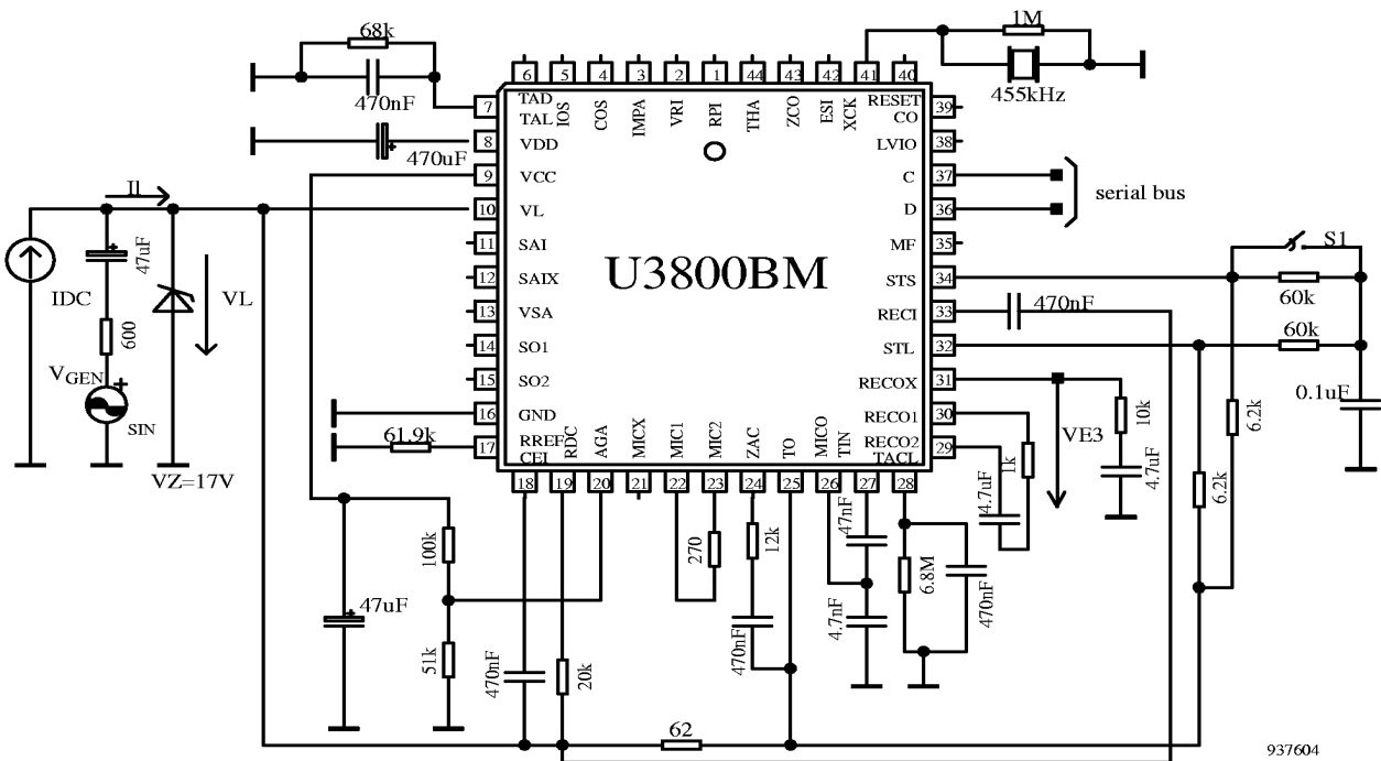
Figure 7. Test circuit
