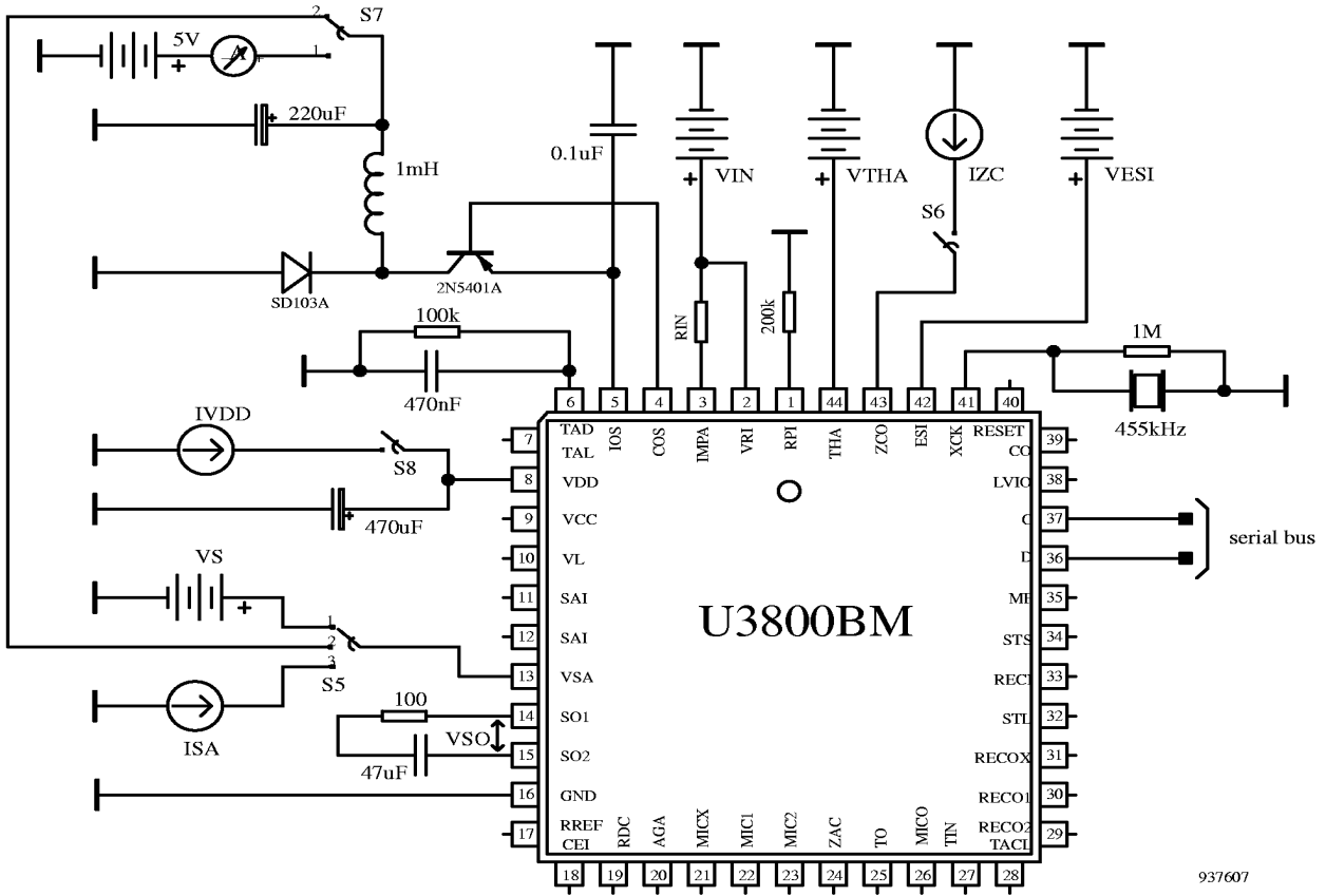
Figure 10. Test circuit
