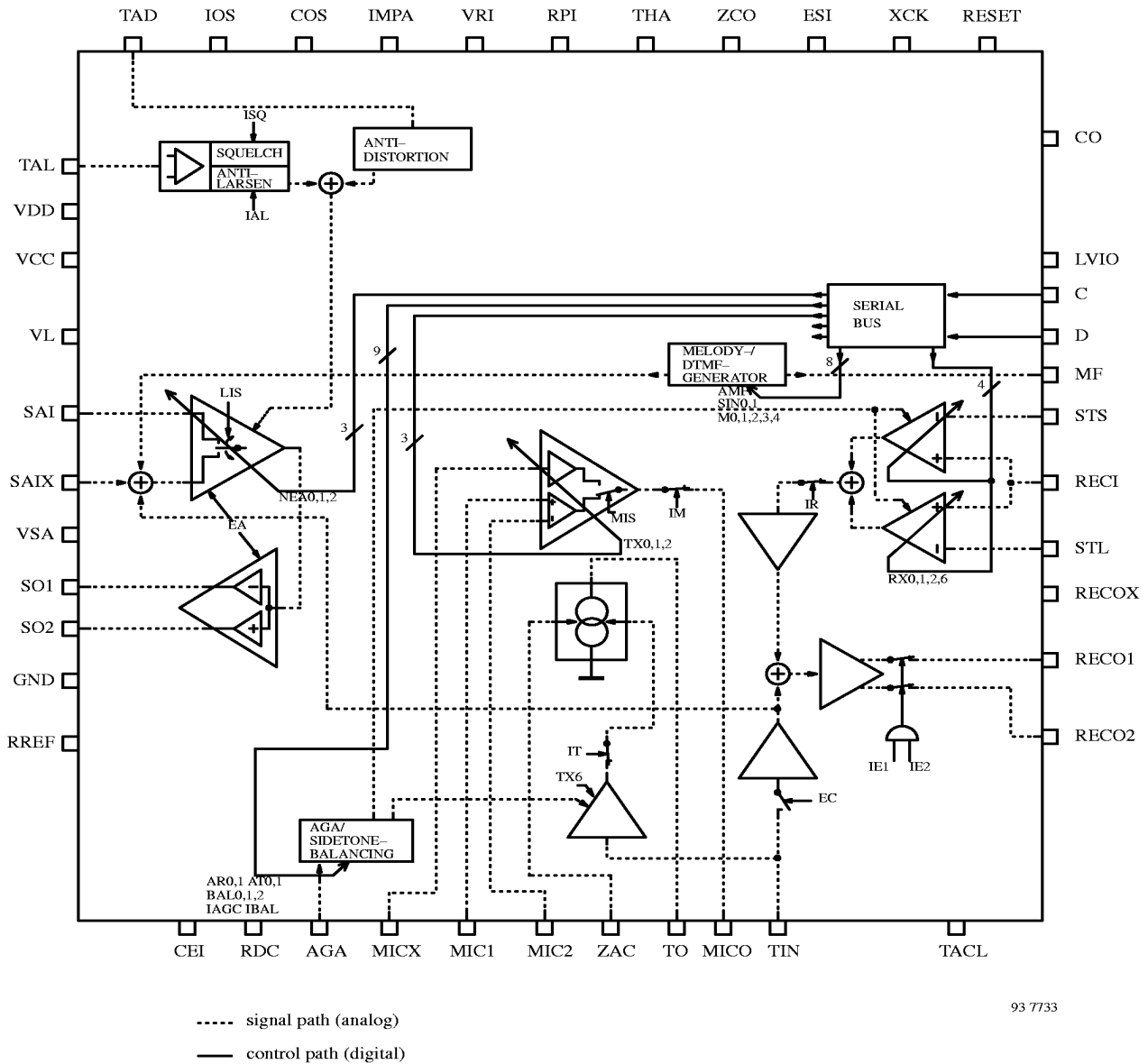
Figure 3. Digital adjustment of the analog parameters by the serial bus microprocessor-interface
