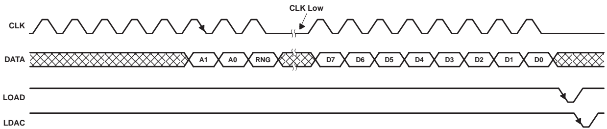
Figure 4. LDAC Controlled Update Using 8-Bit Serial Word
