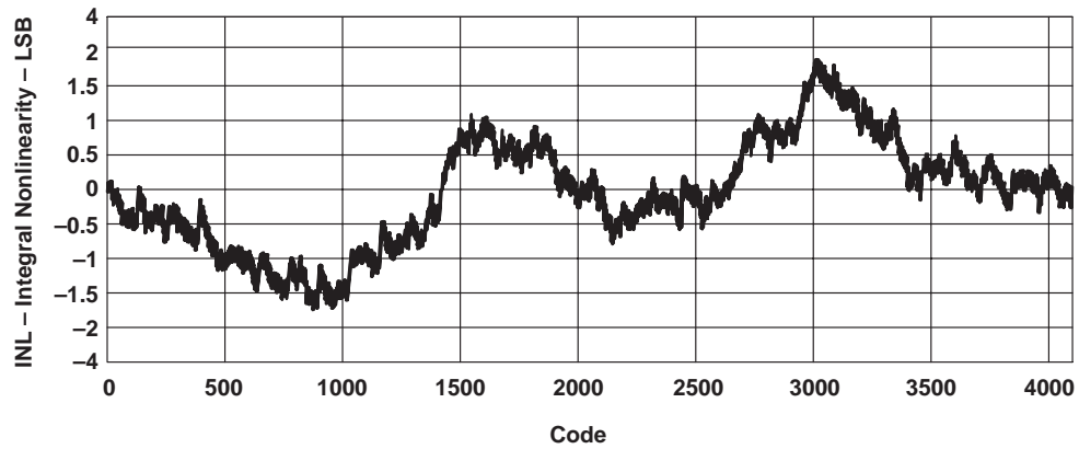
Figure 13. Integral Nonlinearity
