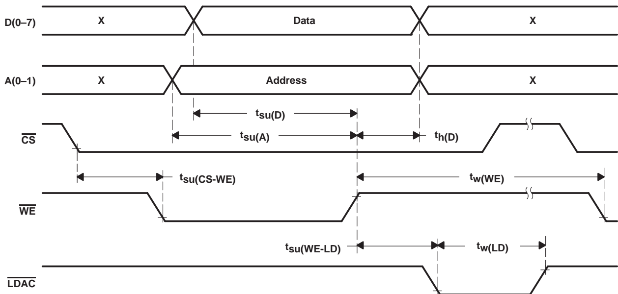
Figure 1. Timing Diagram
