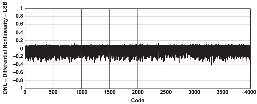
Figure 12. Differential Nonlinearity
