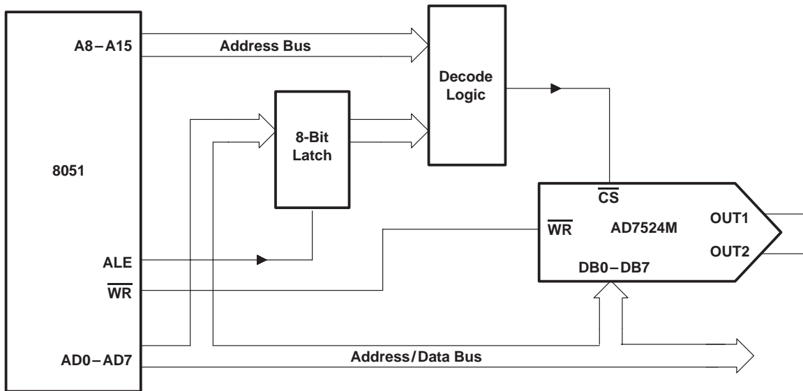
Figure 6. AD7524M-8051 Interface
