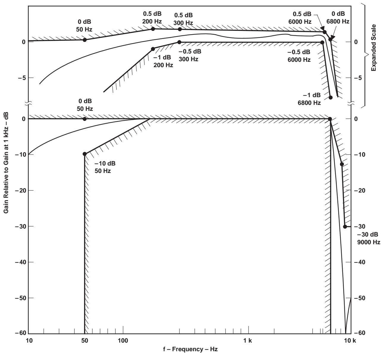
Figure 1. Transfer Characteristics of the Transmit Filter
