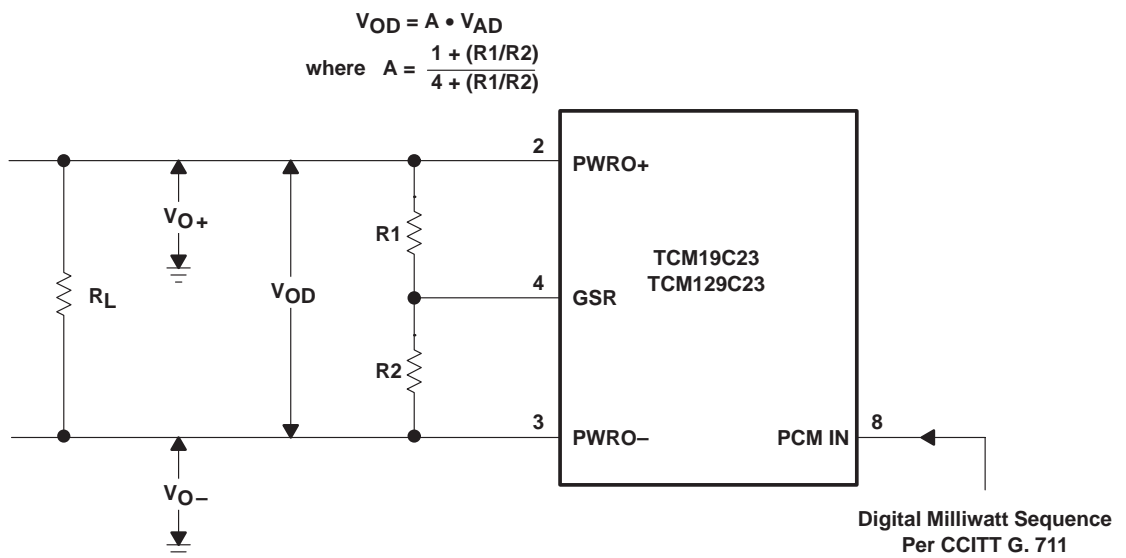
Figure 8. Gain-Setting Configuration
