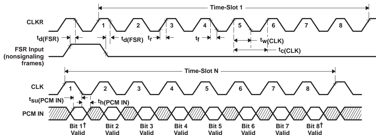
Figure 3. Transmit Timing (Fixed-Data Rate)
